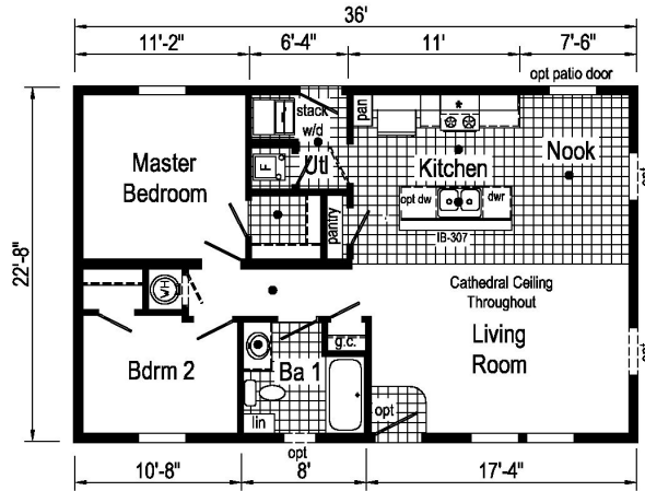
3AM2601-E 2436 Approx. 852 Sq. Ft. ● = Std. can light * = Std 4" staggered overhead cabinets with opt. flat ceiling
